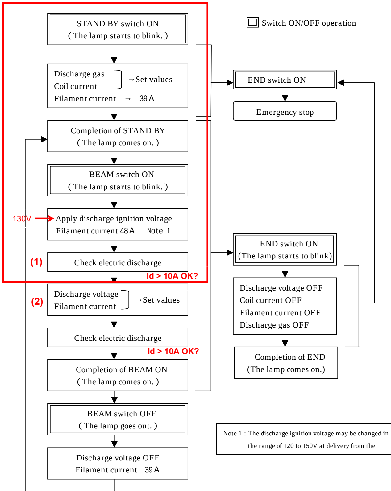
fig.3-7 Performance Chart of the Plasma Source at Semi-auto Control
